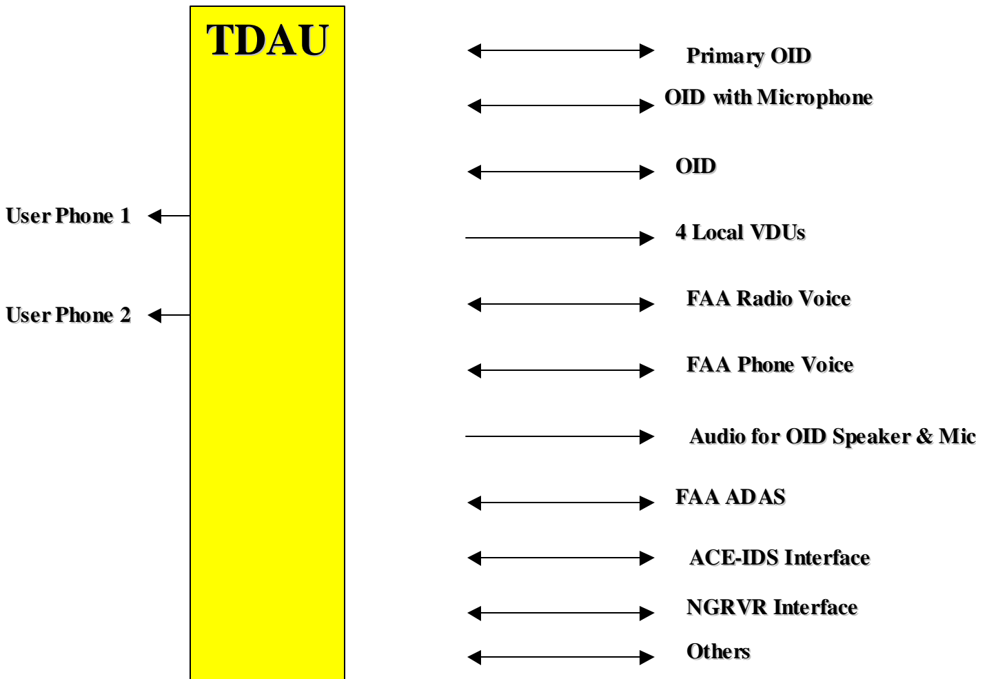
Figure 3.10-1 Communication Ports Functional Configuration
