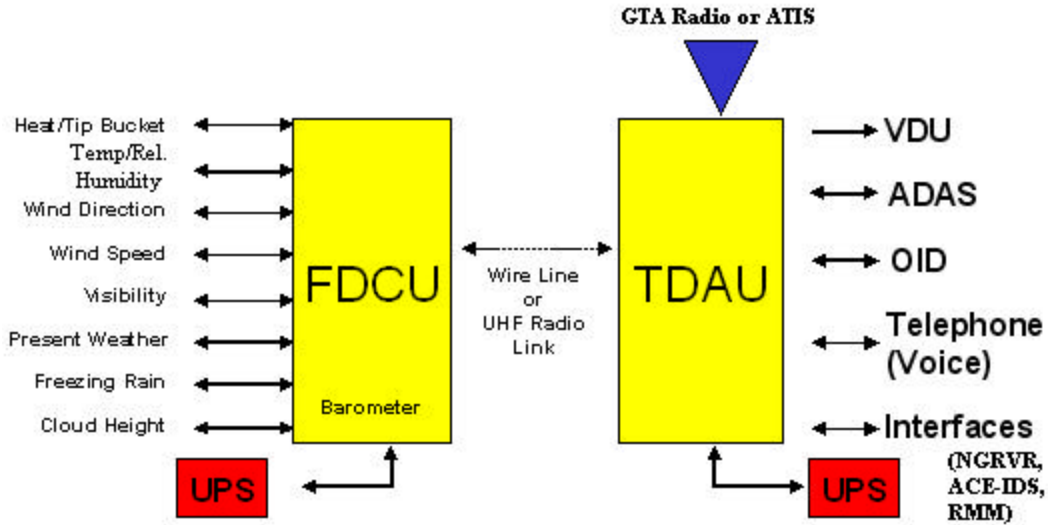
Figure 3.2.1-1 AWSS Block Diagram
