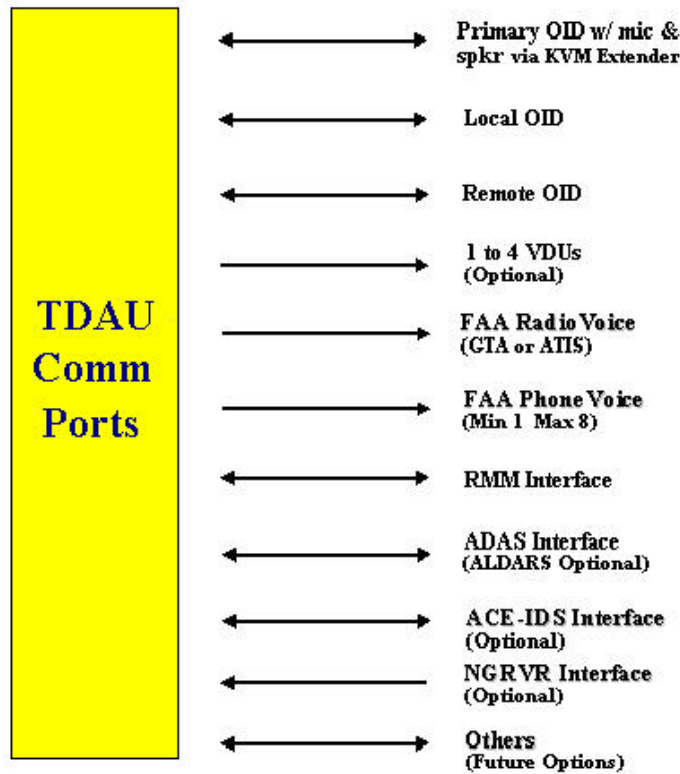
Figure 3.10.1-1 Functional Configuration – TDAU Communications Ports
