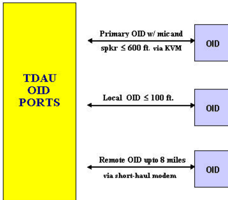
Figure 3.10.3-1 Functional Configuration – TDAU OID Ports
